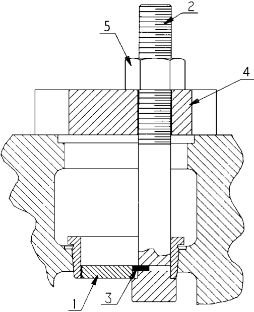
VALVE SEAT PULLER WING GUIDED & GRAVEL TYPE (OPTIONAL EQUIPMENT)
